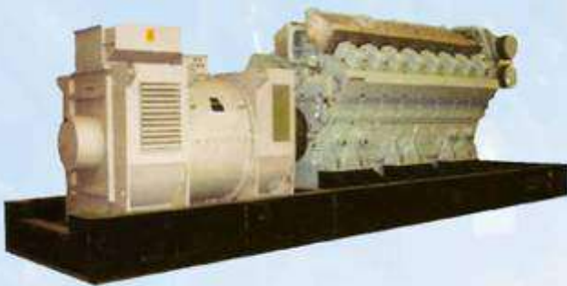
BMGS-16U Open Type (S16U-PTK) Cap: 4100 kVA Prime (50Hz-1000rpm)
